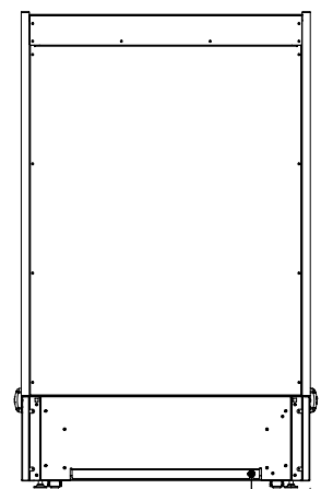
REAR ELEVATION
