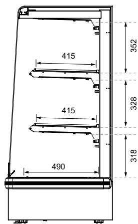
SECTION VIEW
