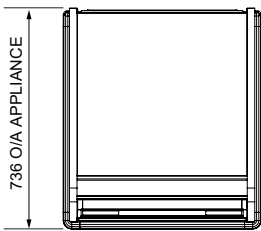
PLAN VIEW
