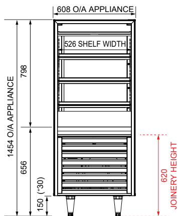
FRONT ELEVATION
