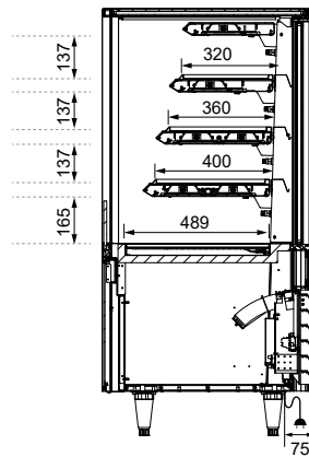
SECTION VIEW
