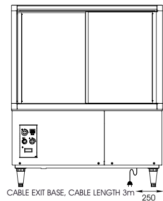
REAR ELEVATION
