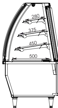
SECTION VIEW
