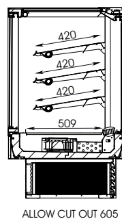
SECTION VIEW
