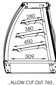
SECTION VIEW
