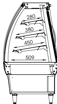
SECTION VIEW
