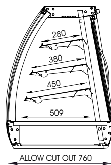
SECTION VIEW
