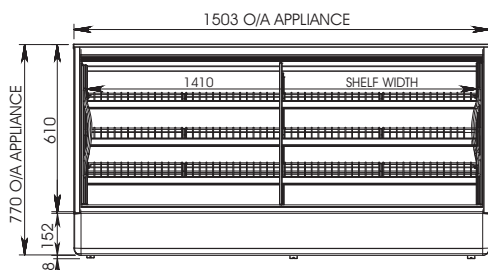
FRONT ELEVATION
