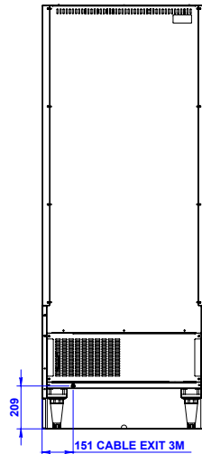
REAR ELEVATION
