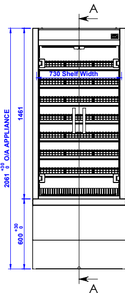
FRONT ELEVATION
