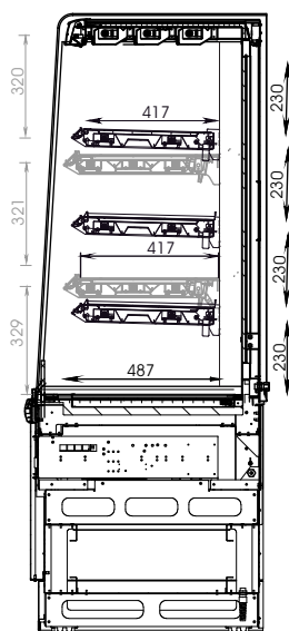
SECTION VIEW
