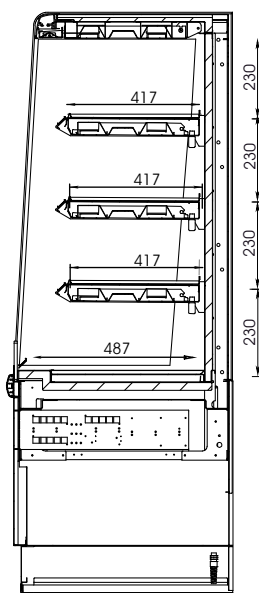
SECTION VIEW
