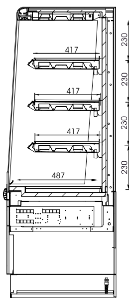
SECTION VIEW
