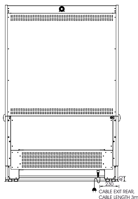
REAR ELEVATION
