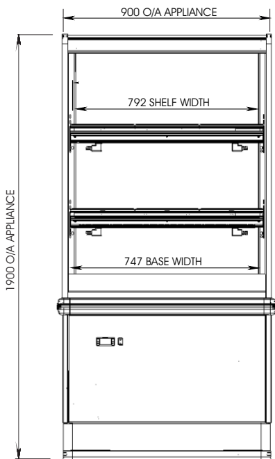
FRONT ELEVATION
