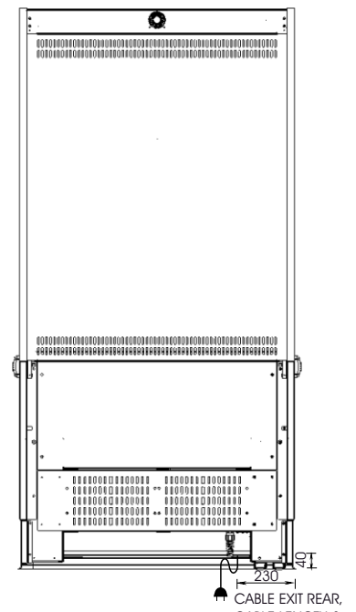
REAR ELEVATION
