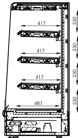
SECTION VIEW
