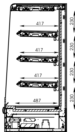
SECTION VIEW
