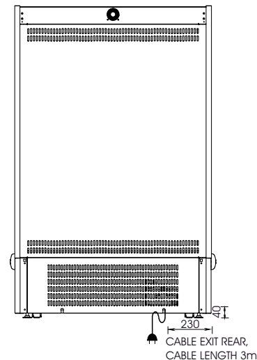
REAR ELEVATION
