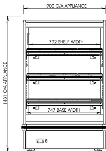
FRONT ELEVATION
