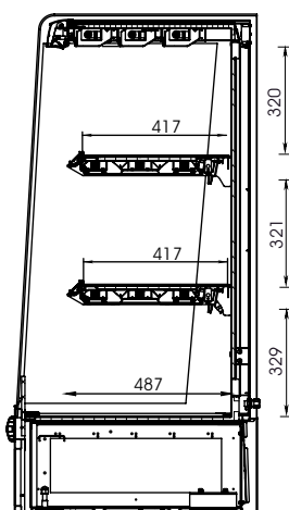
SECTION VIEW
