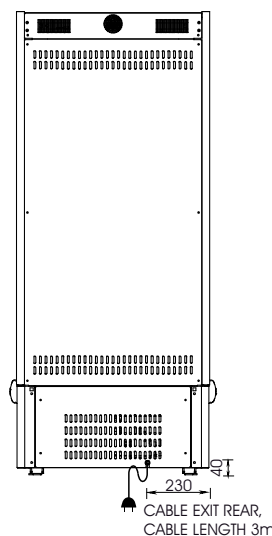
REAR ELEVATION
