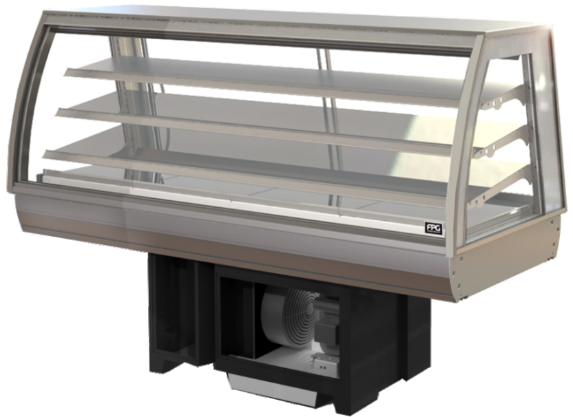
SHOWING : 3000 SERIES REFRIGERATED 1800mm CURVED, WITH FIXED FRONT, IN COUNTER, WITH INTEGRAL CONDENSING UNIT
