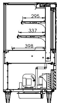
SECTION VIEW
